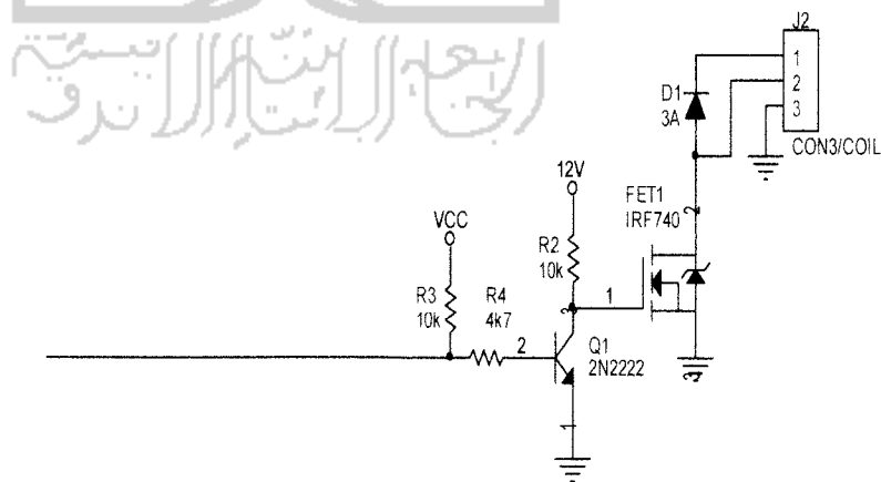
Gambar 3.5. Driver solenoid
