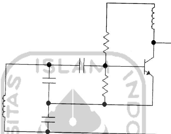
Gambar 3.8 Osilator Colpitts
