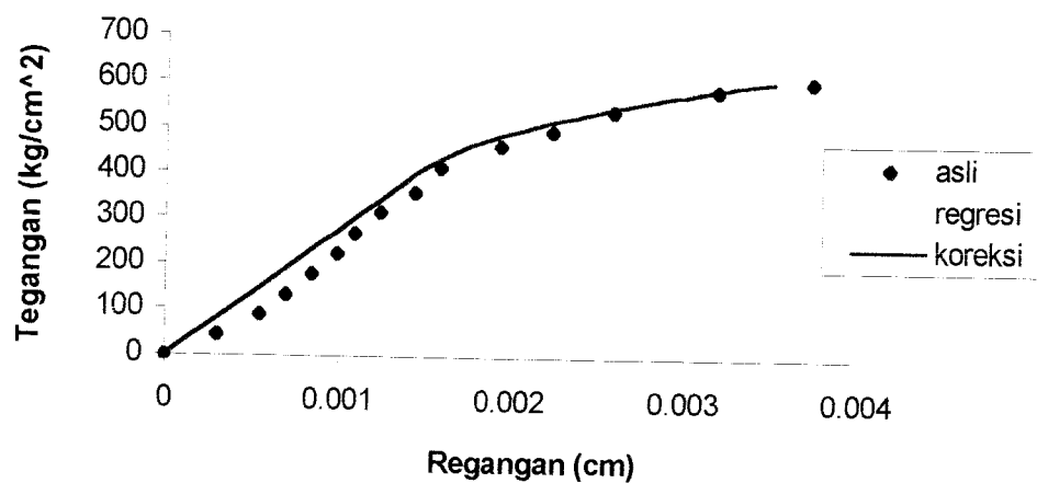
Gambar 5.3 Diagram Tegangan-Regangan Kayu Sampel 3
