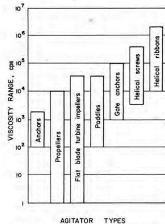
Figure 1-1. Viscosity ranges for agitators.
