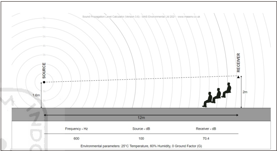
Graphics from noise tool amphitheater to audience Source : Author,2021
