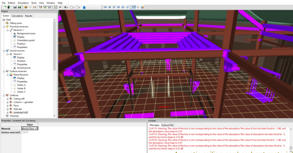
Acoustic ceiling as absorbent material
