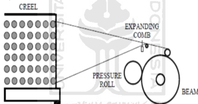
Gambar 3.3 Mesin Direct Warping
