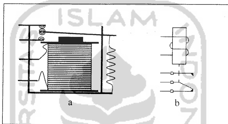
Gambar 2.7 a)Sistem Mekanik Relai b)Simbol Relai
