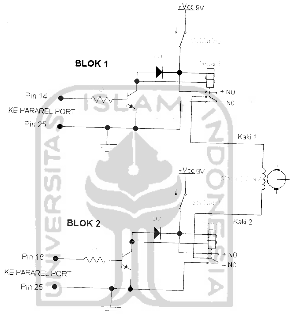
Gambar 3.3 Skema driver
