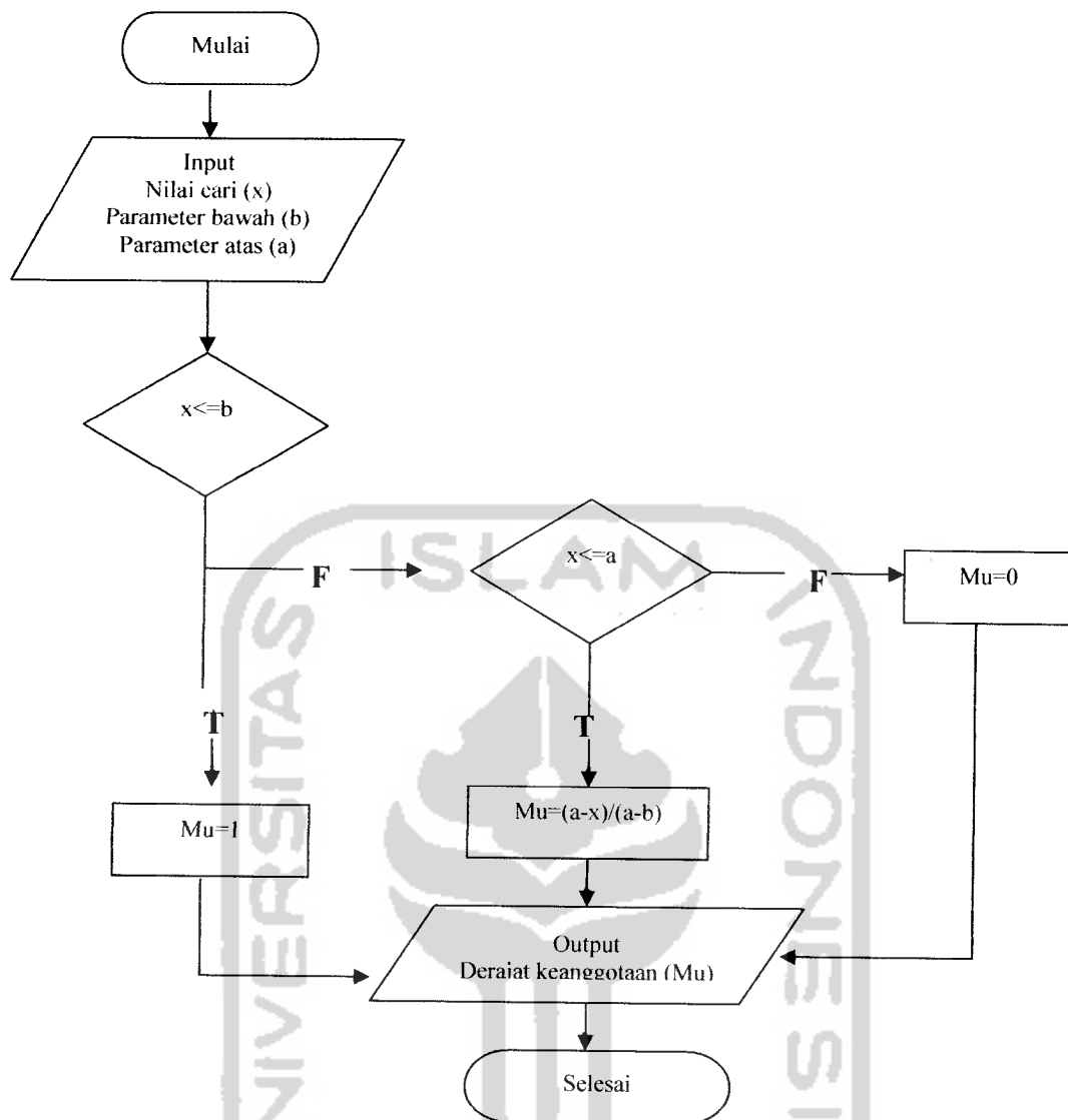
Gambar 3.12 Flow Chart kurva bahu kiri
