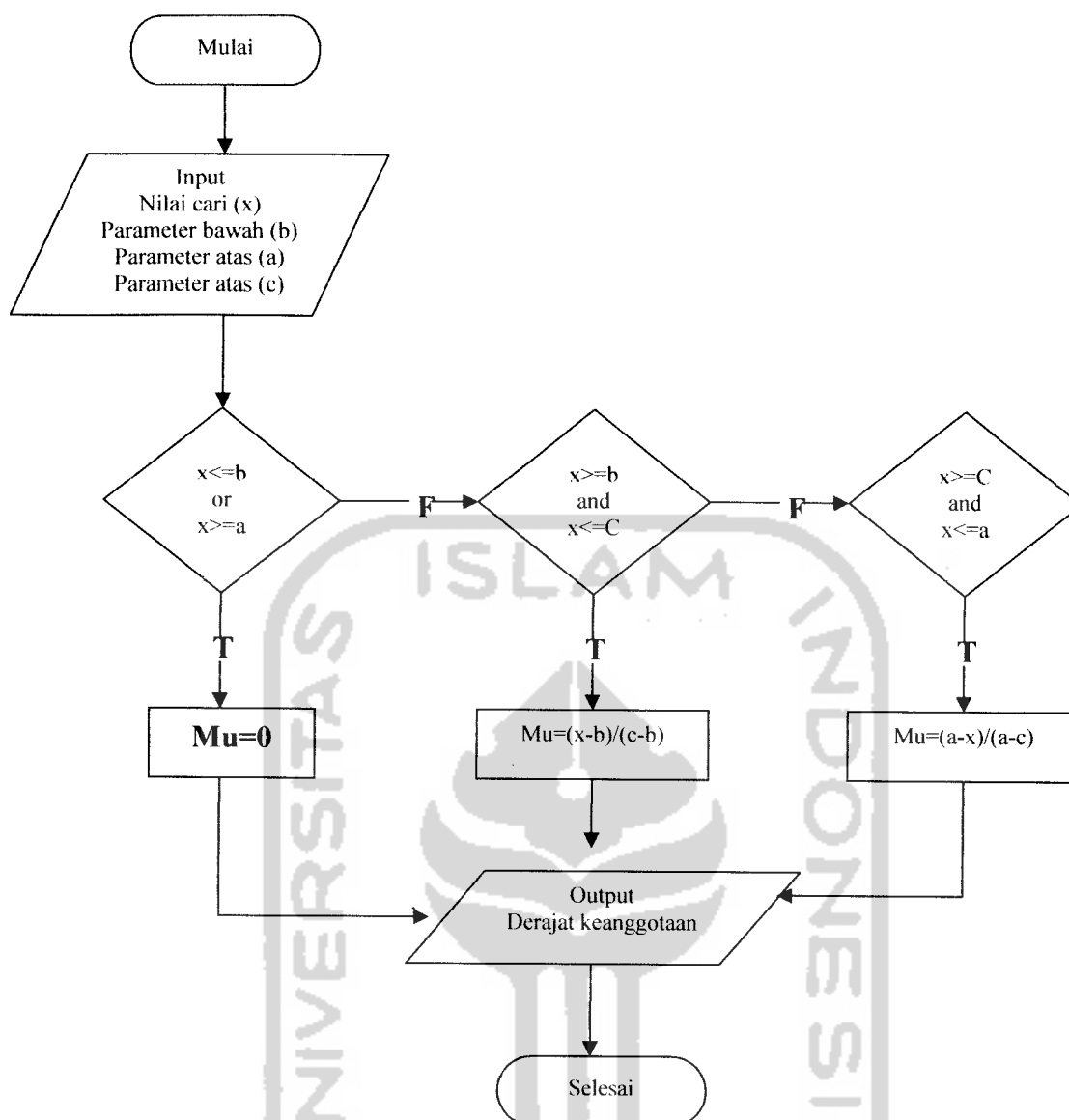
Gambar 3.16 Flow Chart kurva segitiga
