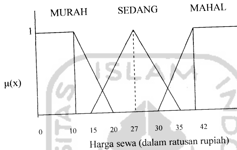
Gambar 3.17 Variabel harga sewa
