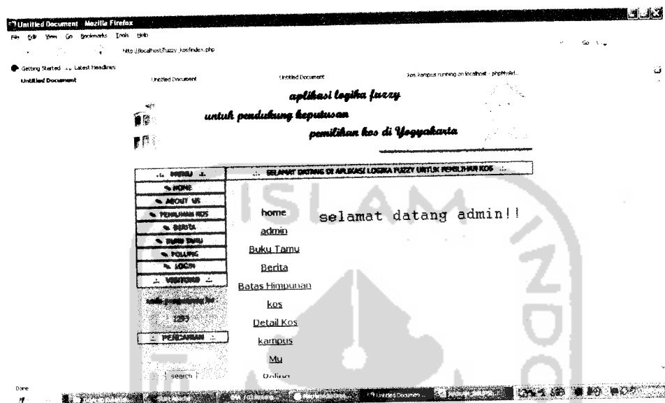
Gambar 3.43 Halaman Administrator
