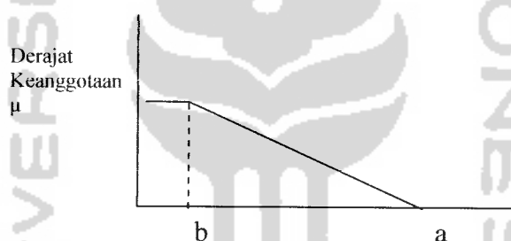
Gambar 3.11 Kurva bahu kiri
