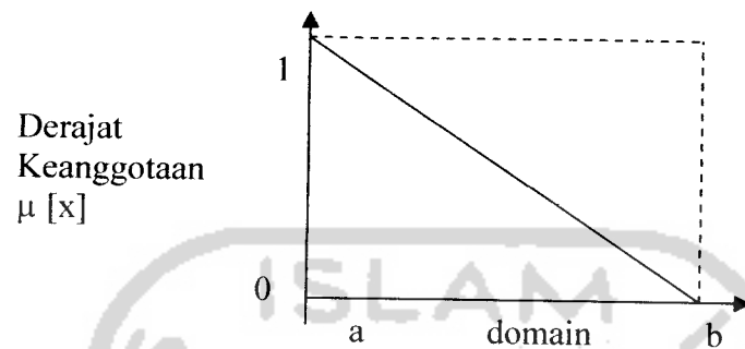
Gambar 2.2 Representasi Linier Turun
