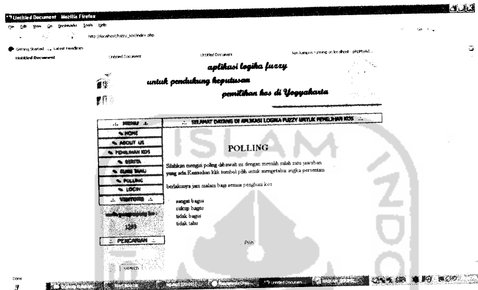
Gambar 3.39 halaman polling
