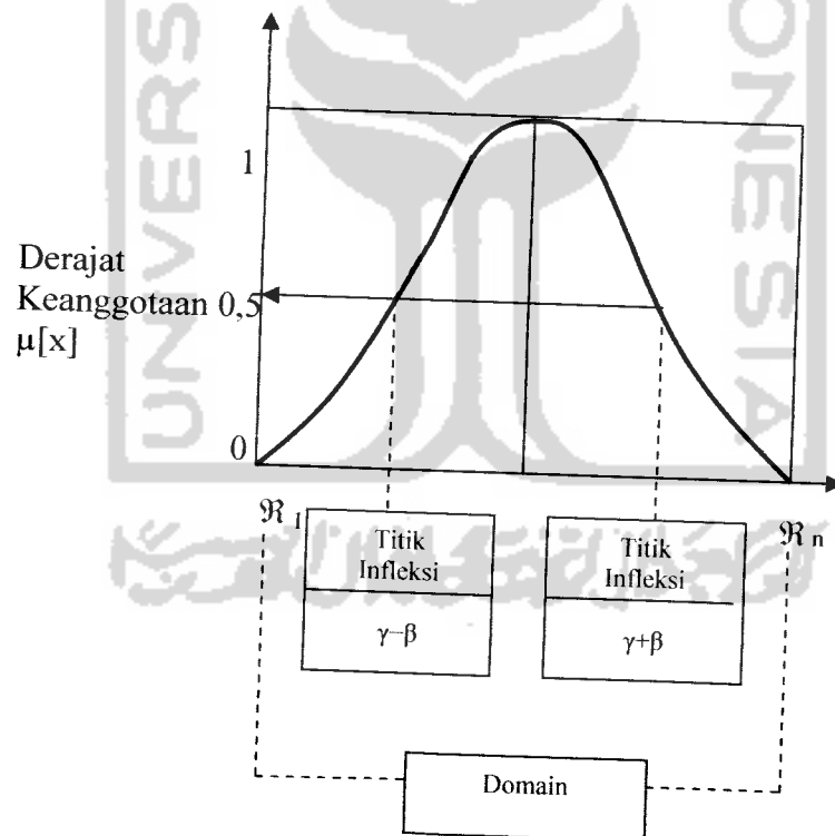
Gambar 2.9 Karakteristik fungsional kurva BETA
