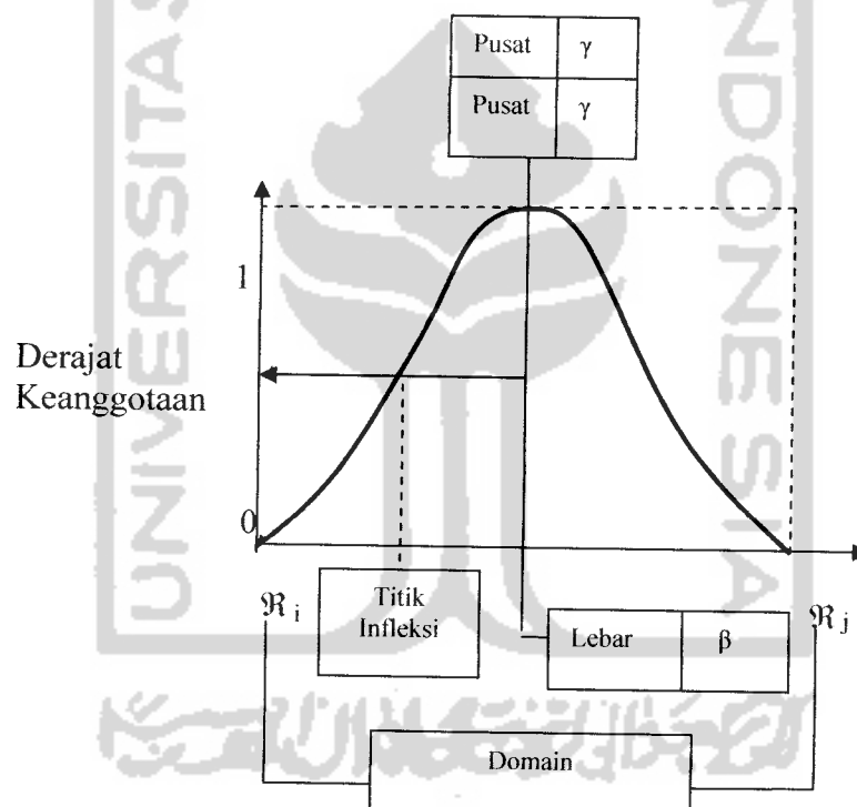
Gambar 2.8 Karakteristik fungsional kurva \pi
