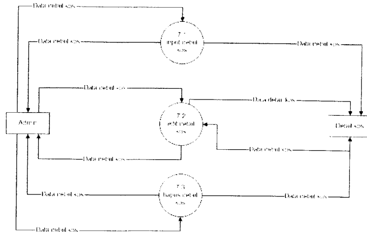
Gambar 3.9 DFD level 2 pengolahan detail kos
