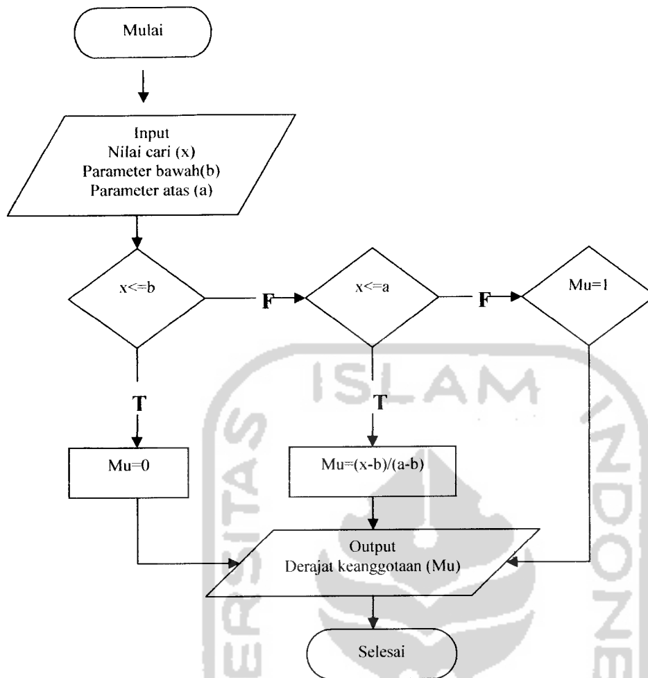
Gambar 3.14 Flow Chart bahu kanan
