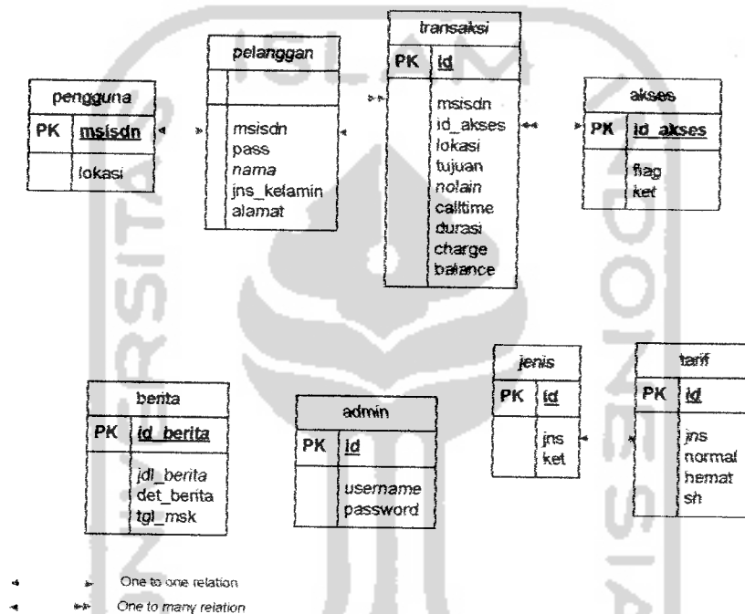
Gambar 3.5 Diagram Relasi Antar Tabel
