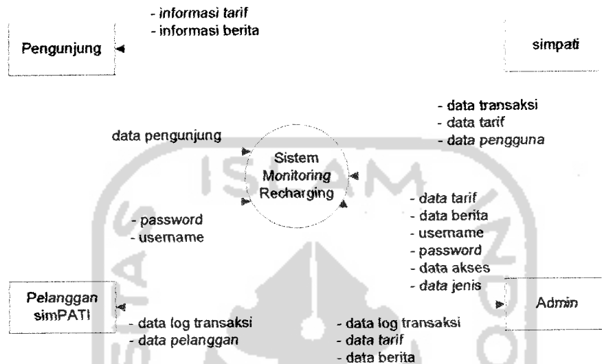
Gambar 3.1 Diagram Konteks WAPsite Monitoring Recharging Perusahaan Telkomsel
