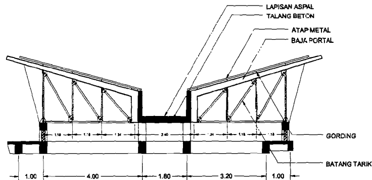
DETAIL ATAP SKALA 1 : 100
