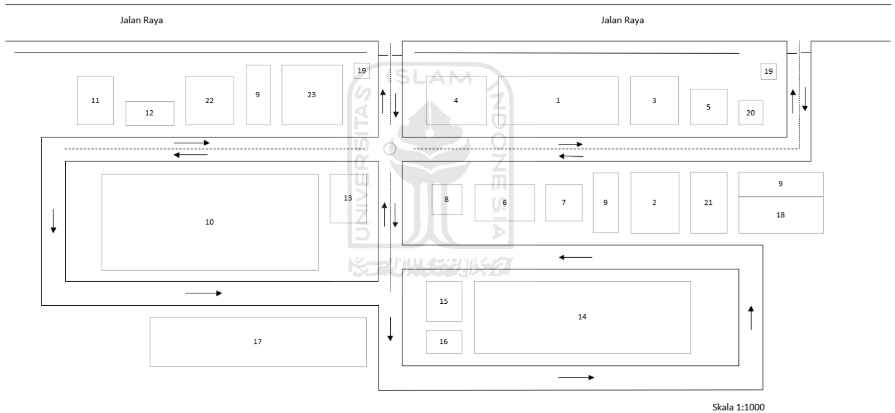
Gambar 4. 2 Layout Pabrik Glukosa
