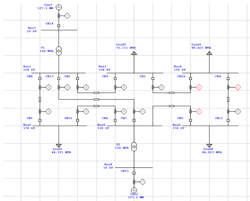
Gambar 3.1 Single line diagram sistem IEEE 8 bus
