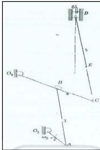
Gambar 2-10 Mesin powell (Holowenko, 1985)
