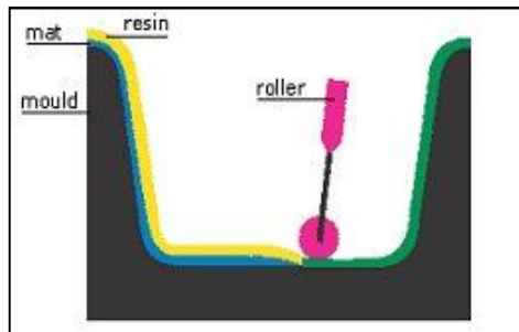
Gambar 3-2 Hand Lay-Up (Ultracki, 1990).
