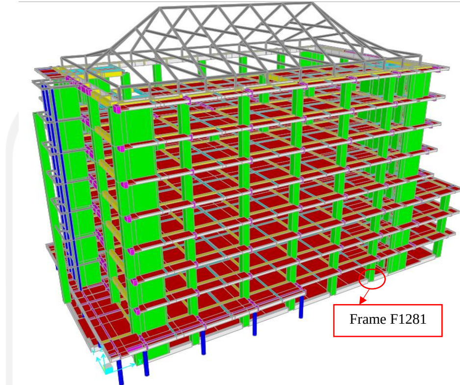
Gambar 5.7 Portal 3D Arah X
