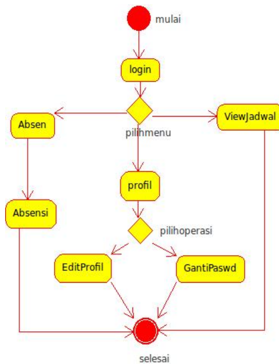
Gambar 3.7 Activity Diagram Mahasiswa
