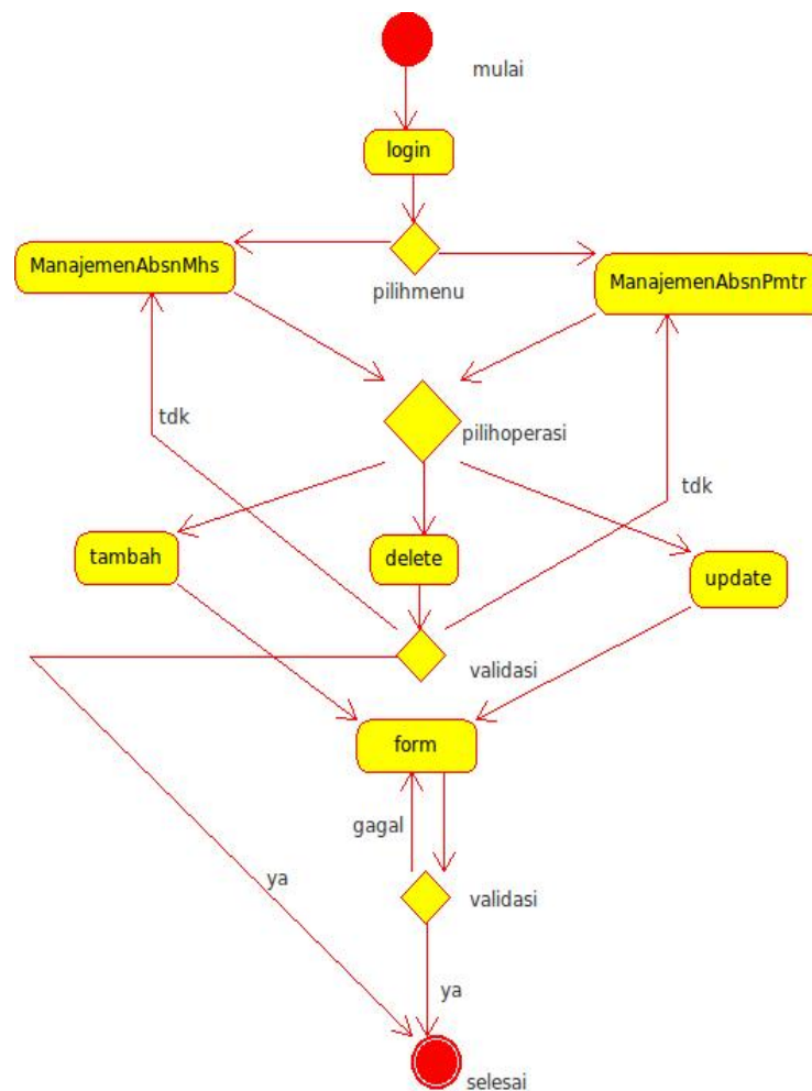
Gambar 3.3 Activity Diagram Manajemen Absen
