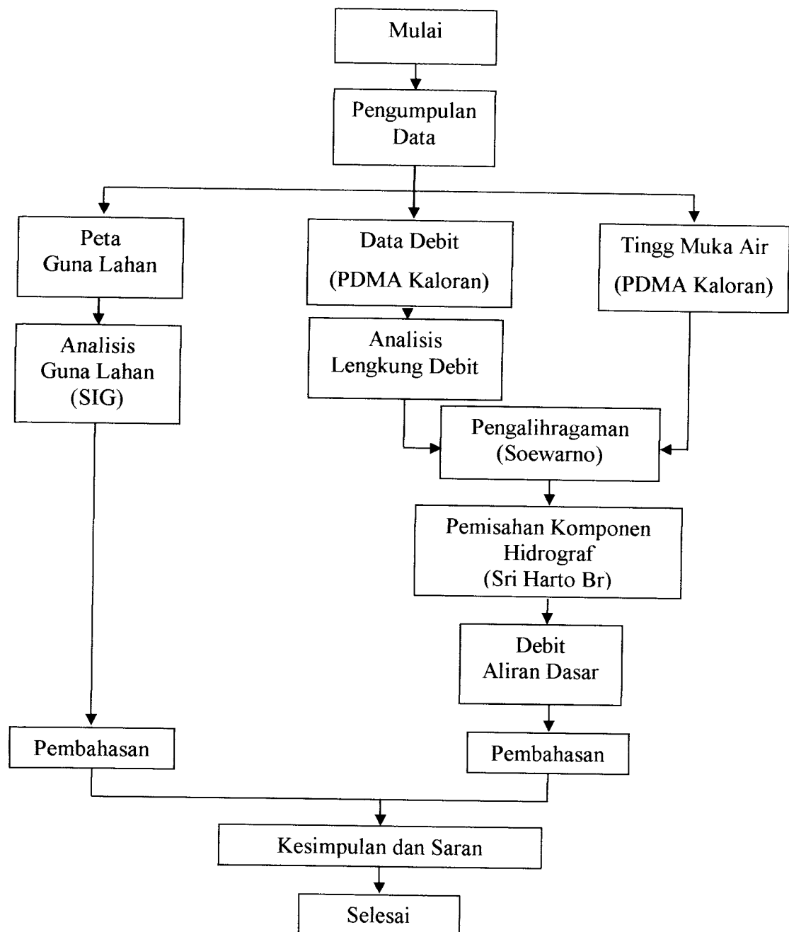
Gambar 4.1 Proses Penelitian
