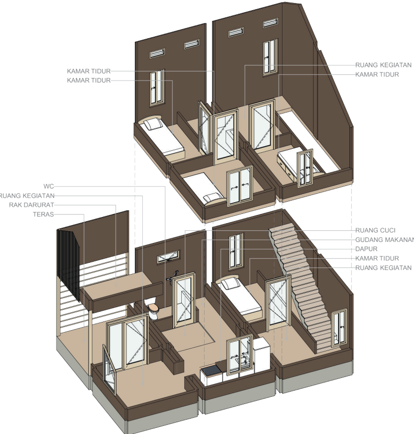
Tipe Extended
