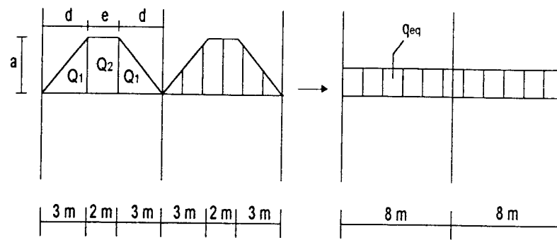
Gambar 4.10. Perhitungan beban merata ekivalen portal A
