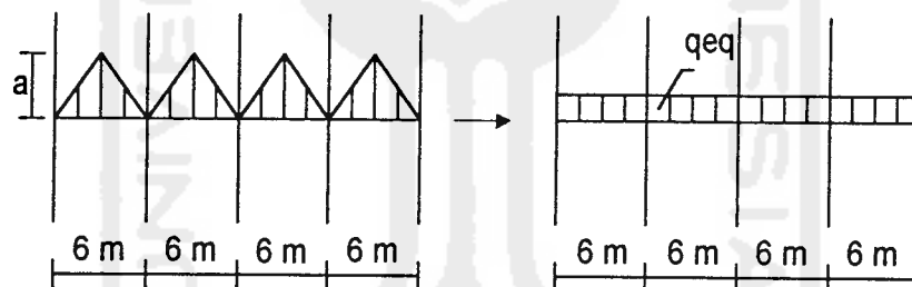
Gambar 4.22. Perhitungan beban merata ekivalen portal III
