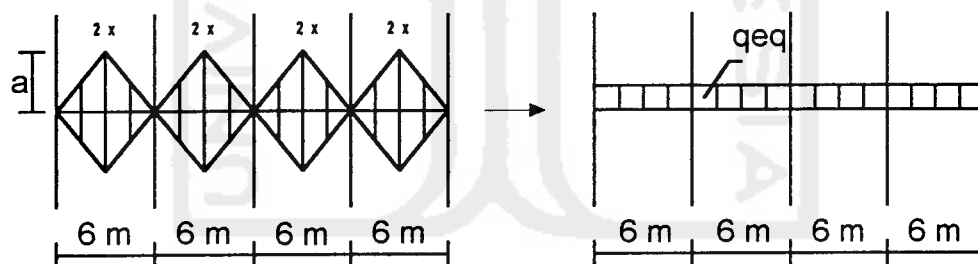
Gambar 4.18. Perhitungan beban merata ekuivalen portal II
