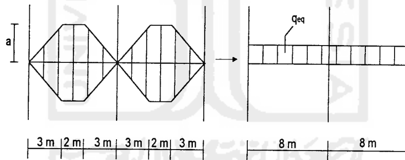
Gambar 4.14. Perhitungan beban merata ekivalen Portal C
