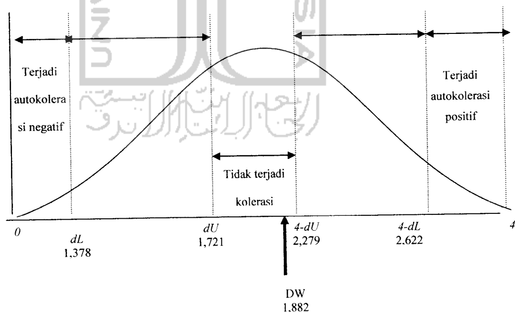
Gambar 4.1. Kurva Durbin Watson
